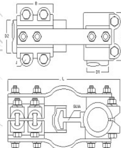
TE TUBO A 2 CABLES TUBO - 1" A 4" CABLE 4/0 AWG A 2000 MCM - TT2C
