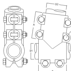
TE TUBO A TUBO 80° - 3/4" A 4" - T80
