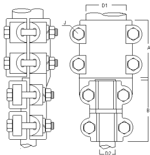
RECTO TUBO A CABLE TUBO 1" A 4" CABLE 2AWG A 2000 MCM - RTC
