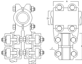
TE TUBO A 2 CABLES TUBO - 1" A 4" CABLE 4/0 AWG A 2000 MCM - TT2CE
