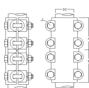
RECTO TUBO A TUBO 1" A 4" - R
