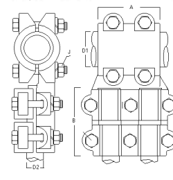
TE TUBO A 2 CABLES TUBO - 1" A 4" CABLE 4/0 AWG A 2000 MCM - TT2C
