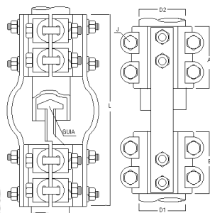
RECTO TUBO A TUBO FLEXIBLE TUBO 1" A 4" - RTTF
